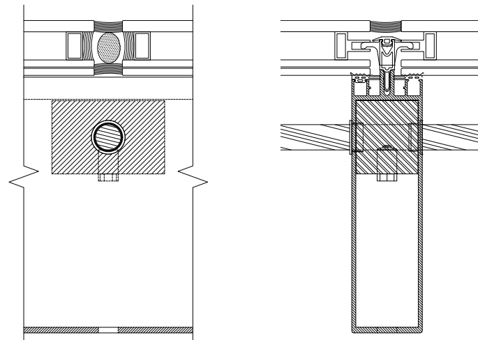
Glass Wall Detail
