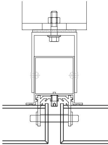
Aluminum Composite Panel Detail
