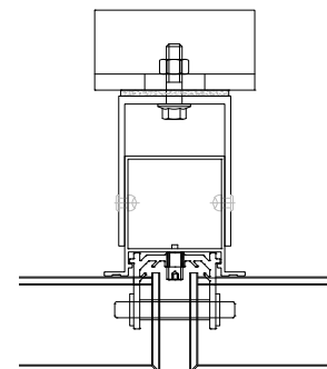
Aluminum Composite Panel Detail
