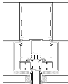
Curtain Wall Detail
