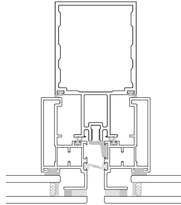
Curtain Wall Detail
