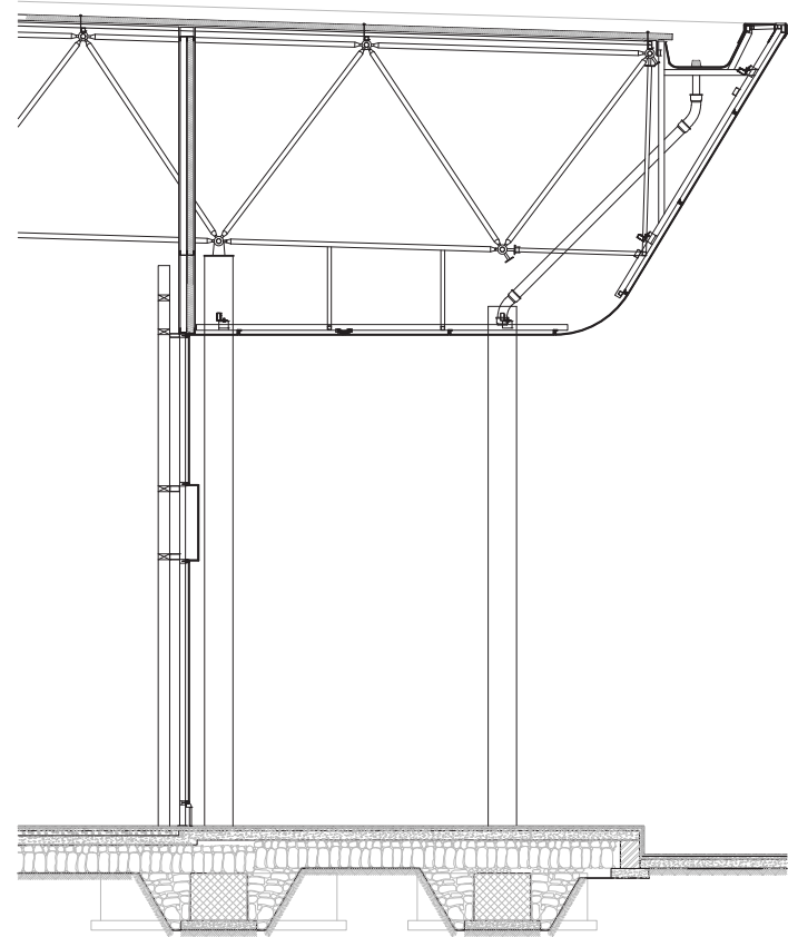
Vertical Section
