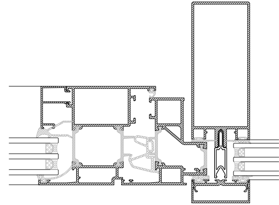
Curtain Wall & Side Hinge Doors Detail
